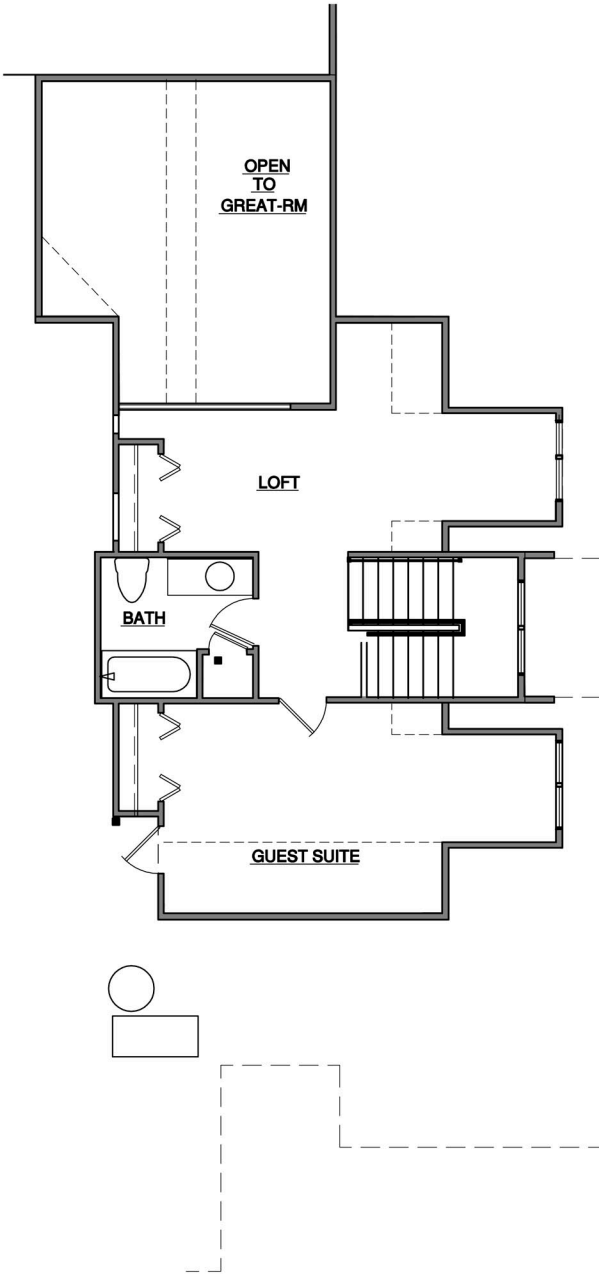
Second Floor Plan Option 'A'
